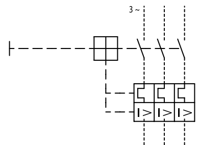
Three-phase operation
