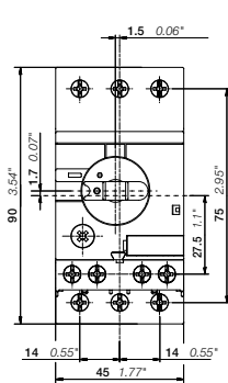
MS116 ≤ 16 A
