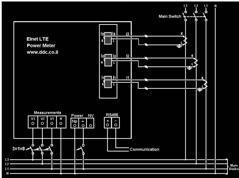
Figure 3.2 – Wiring Diagram
