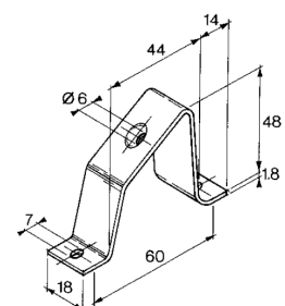
Mounting Bracket
