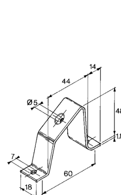
Mounting Bracket
