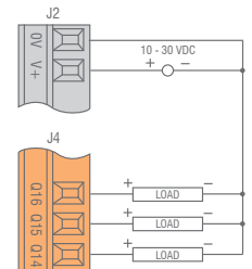
Orange - Positive Logic Digital Out
