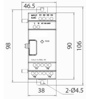
Expansion Modules
