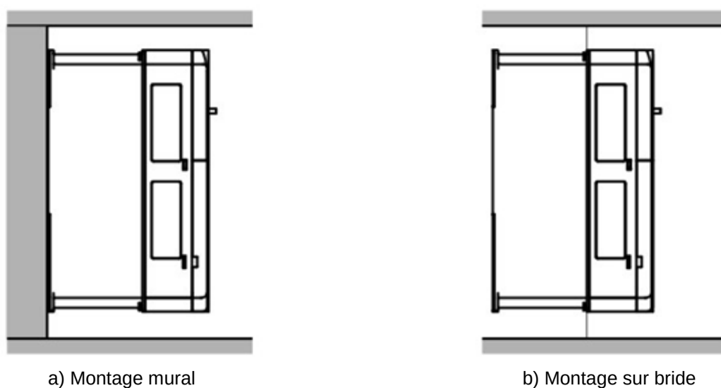
Figure 3-2 : Installation
