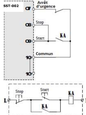
Control mode of relay
