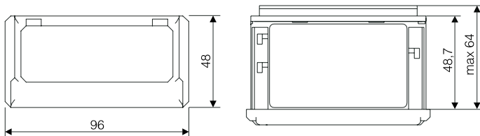
Fig. 2. Overall dimensions
