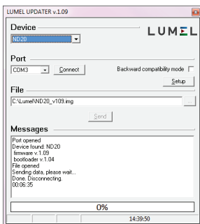
Fig. 13. Program view: a) LPCon, b) updating of software
