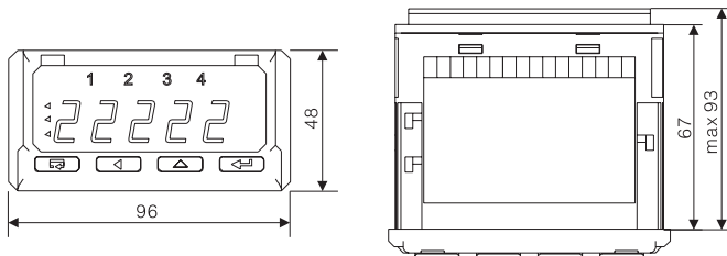
Fig. 3. Overall Dimensions
